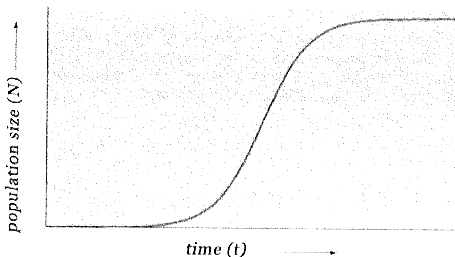
Figure 1. A typical logistic curve used in stock recruitment models. Initially, a population at low densities undergoes exponential growth, eventually population growth is increasingly constrained as carrying capacity is approached.
